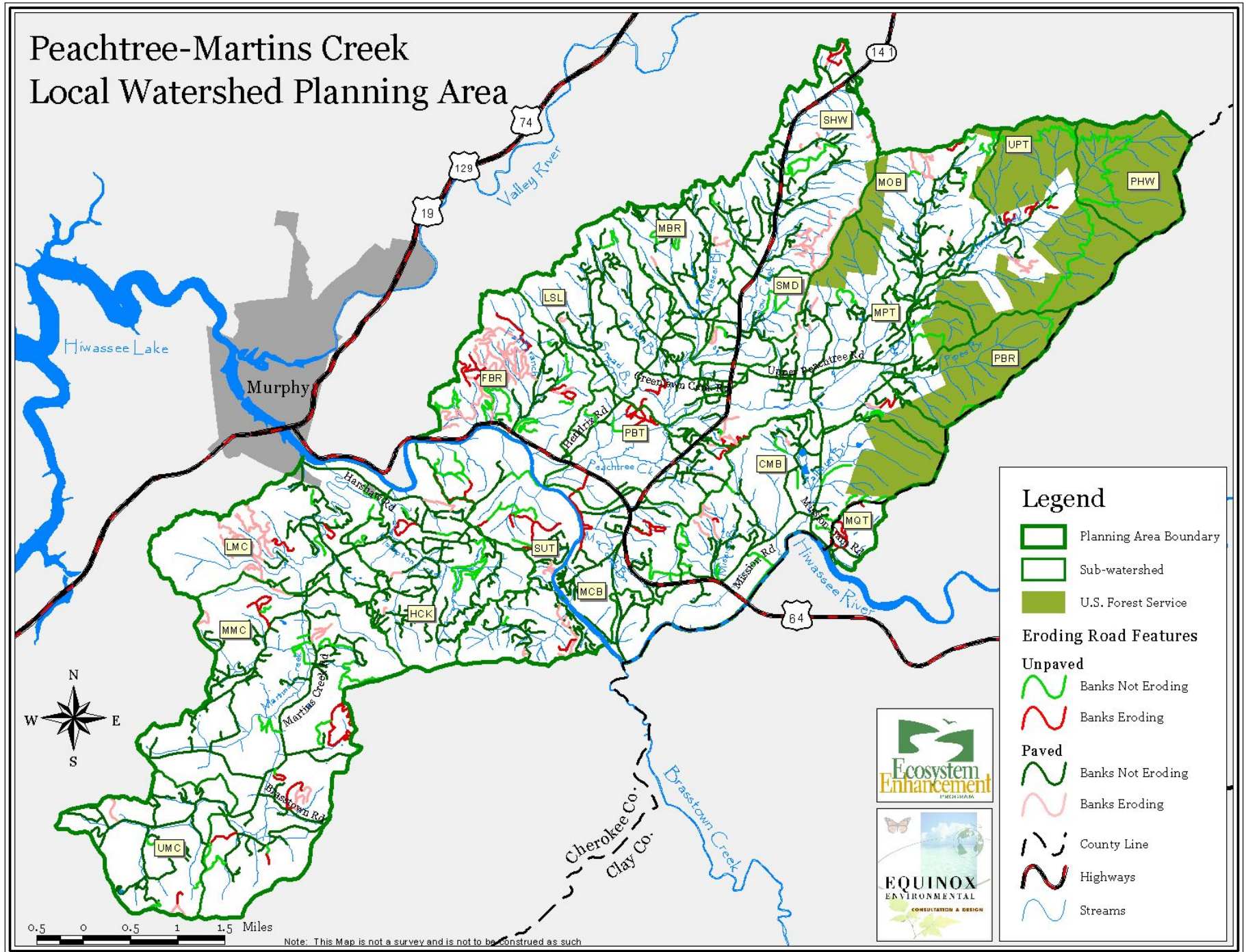
Figure A7 Road Surface Type and Location of Eroding Road Banks and Ditches (IPSI Database, TVA)
